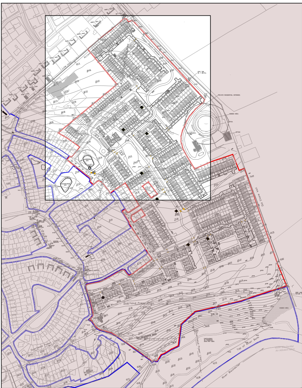
Proposed Site Layout - Key Plan Scale : 1:5000
