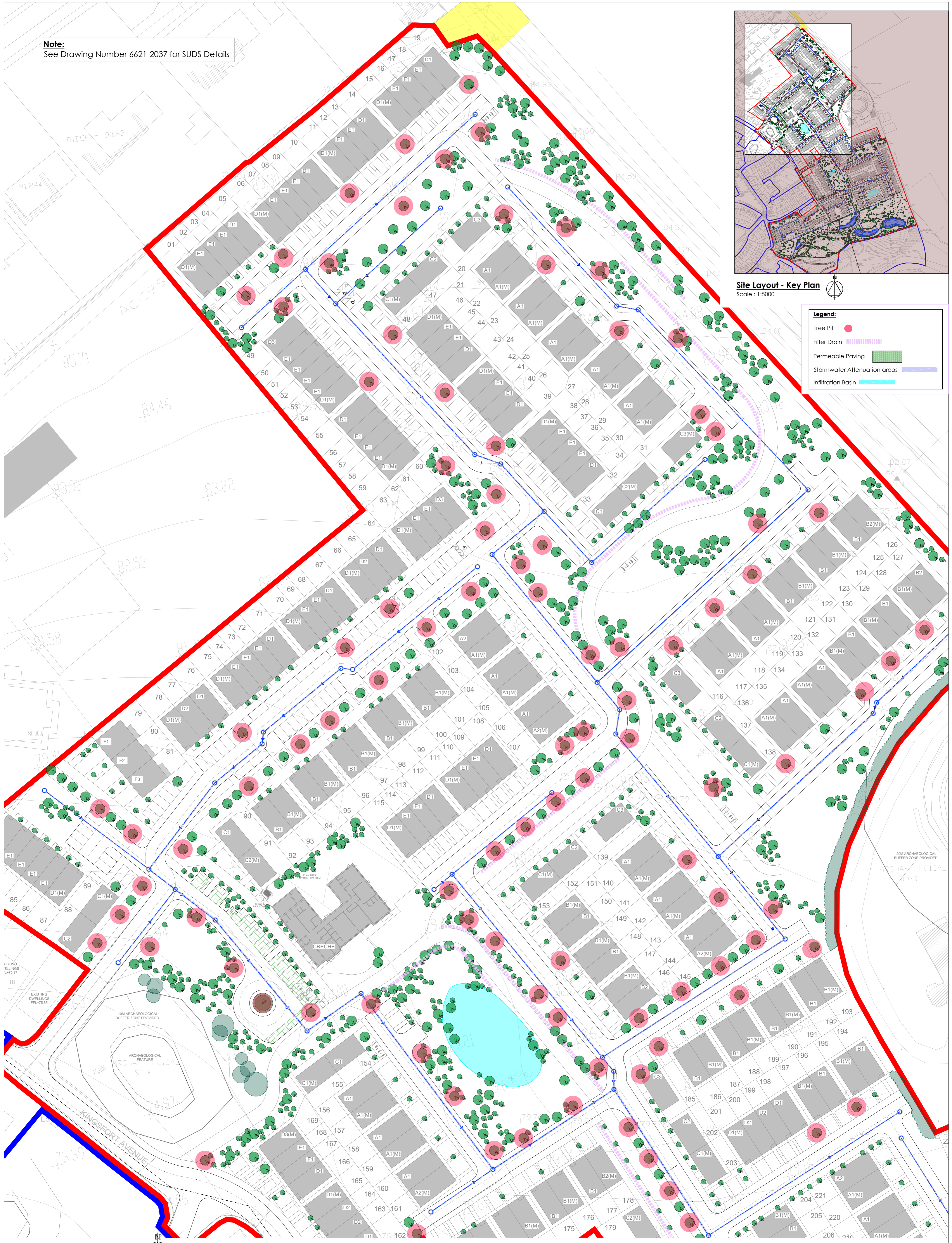
Proposed SUDS Layout 1 of 3 Scale : 1:500
