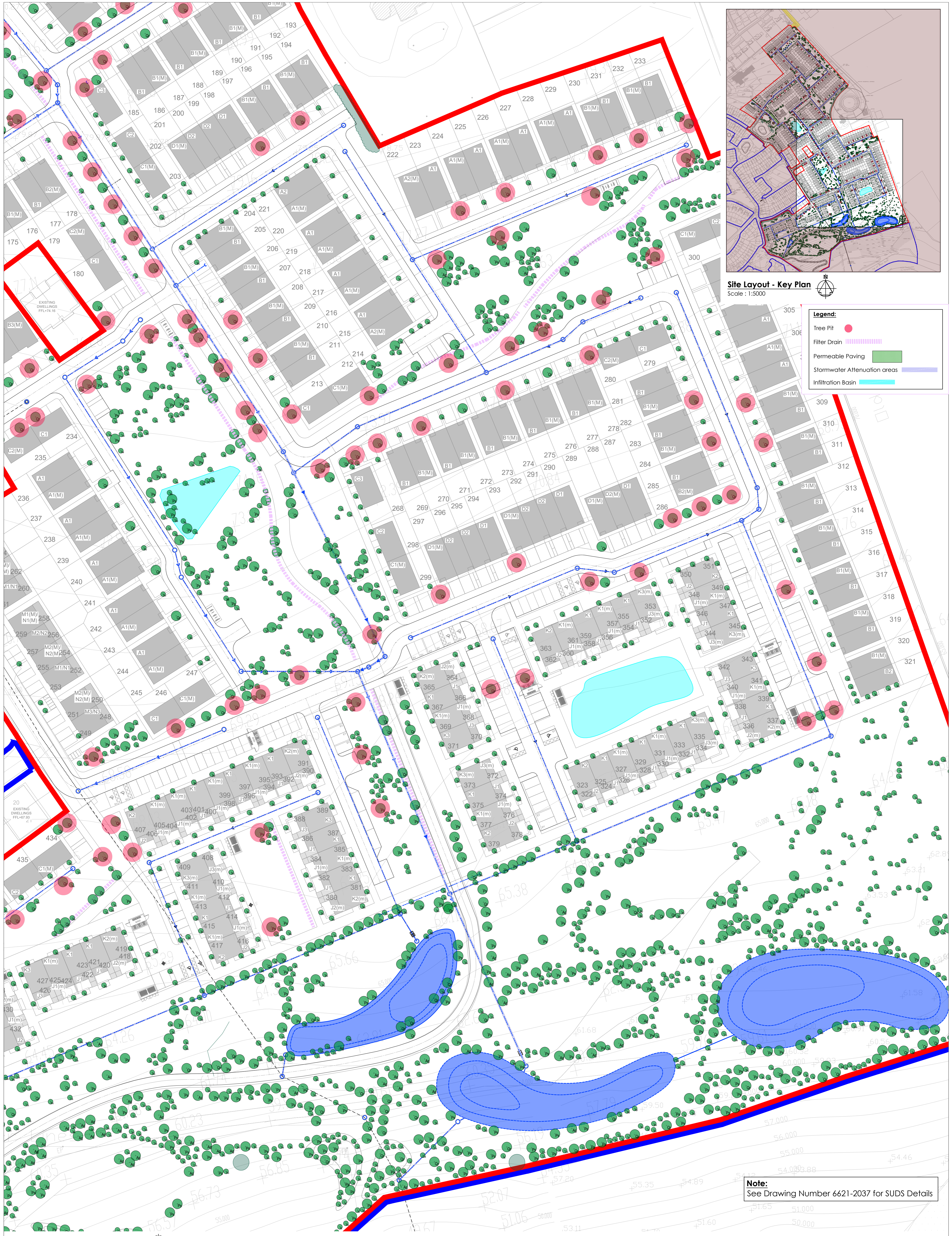
Proposed SUDS Layout 2 of 3 Scale: 1:500
