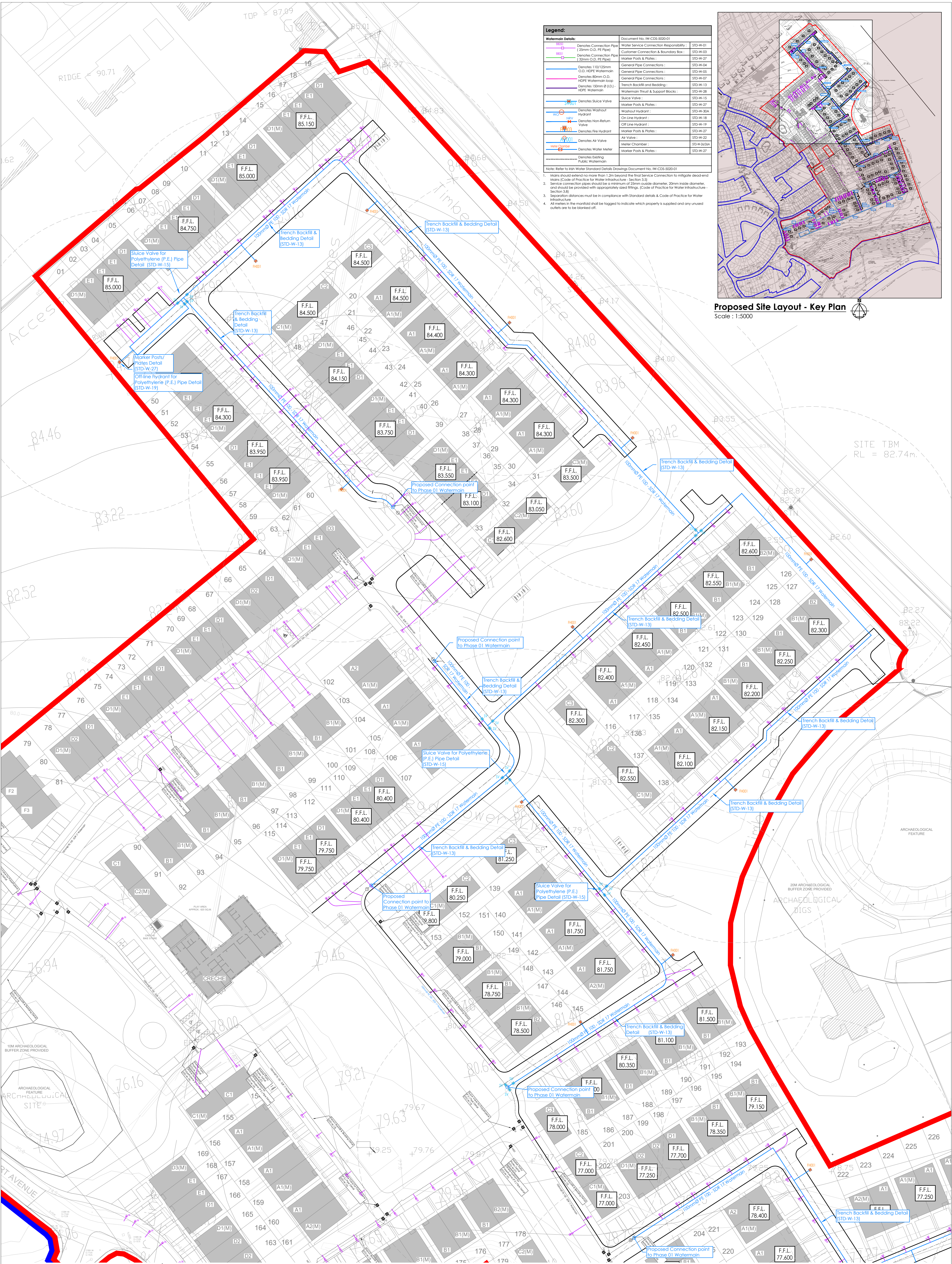
Proposed Watermain Layout 1 of 3 Scale: 1:5000
